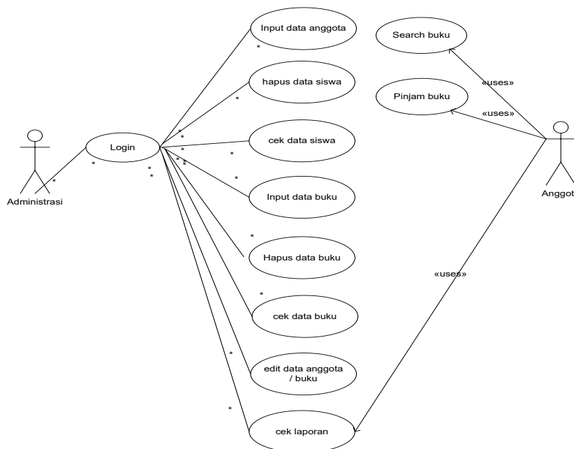
Gambar 4 Use Case
